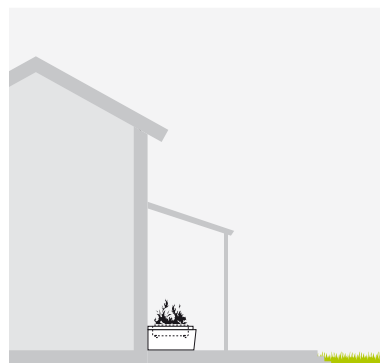
inserto braciere, installazione esterna gas fire logs insert, outdoor installation
